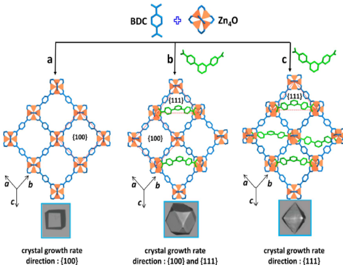
Fig. 3 Cubic crystal shape (a) is governed by the slower rate of crystal growth in the direction of faces. Additive ( m -terphenyl-4,4-dicarboxylate indicated in green) blocking MOF-5 growth along the \{111\} direction partially or completely at the expense of all \{100\} facets during crystal growth in creation of cubooctahedral (b) and octahedral (c) crystal morphologies. Reproduced from Suresh et al. 52 with permission from American Chemical Society, copyright 2021.
