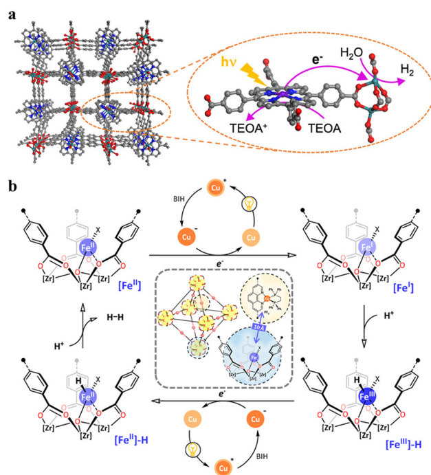
Fig. 8 (a) Schematic representation of the Ru-TBP (Zn) crystal structure assembled from metalloporphyrin-centered tetracarboxylate and Ru(III) 2 paddlewheel (SBU), showing the visible light-driven HER. Photoexcited porphyrin ligands inject electrons to adjacent Ru 2 SBUs to reduce protons to hydrogen. Subsequently, the oxidized porphyrin ligands are reduced by sacrificial TEOA to regenerate the photocatalytic system. Adapted with permission from ref. 120. Copyright 2018, the American Chemical Society. (b) Sequentially installed Cu(I)-PS and Fe(II)-CAT in Zr 6 -mPT to afford Fe(II)-X@Zr 6 -Cu (X = Br - , Cl - , AcO - , and BF 4 - ) and proposed photocatalytic cycle for H 2 evolution. Adapted with permission from ref. 71. Copyright 2020, the American Chemical Society.
