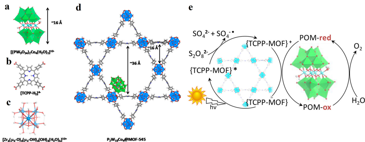
Fig. 13 POM@MOF-545 components: (a) \text{P}_2\text{W}_{18}\text{Co}_4 POM; (b) TCPP- \text{H}_2 linker; (c) Zr-based unit; and (d) \text{P}_2\text{W}_{18}\text{Co}_4 @MOF-545. (e) Schematic representation of the proposed mechanism for the light-driven OER by \text{P}_2\text{W}_{18}\text{Co}_4 @MOF-545. Adapted with permission from ref. 124. Copyright 2018, the American Chemical Society.
