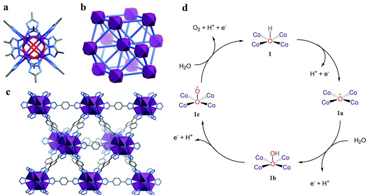
Fig. 12 (a) \text{Co}_8(\mu_4\text{-OH})_6(\text{Rtrz})_{12} cluster ( \text{Rtrz}^- = 1,2,3\text{-triazolate} group), (b) network topology (octanuclear clusters: violet polyhedra and bistriazolate ligands: blue sticks), and (c) 3D coordination framework ( \text{CoN}_3\text{O}_3 units: violet polyhedra) of MAF-48 (hydrogen atoms are omitted for clarity). (d) Proposed reaction mechanism for using MAF-48 as CAT for light-driven water oxidation. Adapted with permission from ref. 165. Copyright 2019, the Royal Society of Chemistry.
