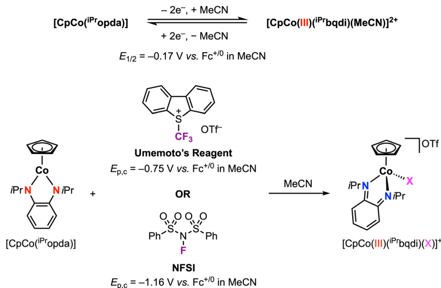
Scheme 6 Stoichiometric \text{Co}^{\text{III}}\text{-X} bond formation ( \text{X} = \text{CF}_3 or \text{F} ) promoted by the phenylenebiquinone redox-active ligand. 49
