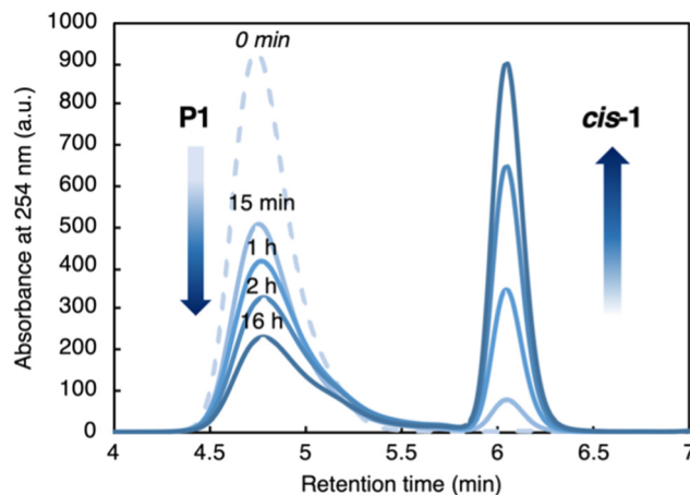
Fig. 4 SEC elograms of recovered P1 over time ([ P1 ] = 0.75 mg mL -1 , THF, RT). See Table 1 for molecular weight characteristics of recovered P1 .
