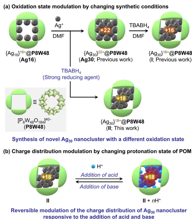
Fig. 1 Diagram illustrating the modulation of electronic states in \text{Ag}_{30} nanoclusters within a ring-shaped POM. (a) Modulation of oxidation states in \text{Ag}_{30} nanoclusters through variations in synthetic conditions. (b) Modulation of charge distribution via protonation and deprotonation of the ring-shaped POM.
