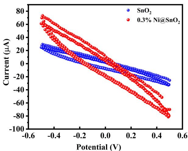
Fig. 14 C–V measurement of pristine \text{SnO}_2 and 0.3% \text{Ni@SnO}_2 samples.
