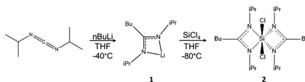
Fig. 2 Preparation of intermediate complex lithium ( N,N' -diisopropylbutylamidinate) (1). Its reaction with silicon tetrachloride forms the complex bis( N,N' -diisopropylbutylamidinate) dichlorosilane (2).
