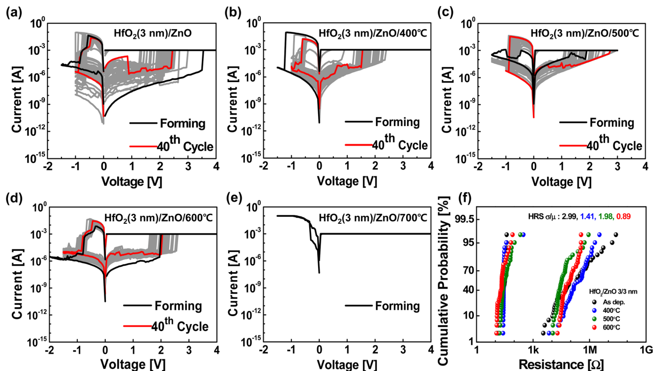
Fig. 5 Typical current–voltage ( I – V ) resistive switching behavior of bilayer HfO 2 /ZnO synaptic devices (a) without and with thermal annealing at (b) 400 °C, (c) 500 °C, (d) 600 °C, and (e) 700 °C for 1 h in a N 2 ambient. (f) Distribution and cumulative probability of the high-resistance state (HRS) and low-resistance state (LRS) in 40 consecutive I – V sweeps for bilayer HfO 2 /ZnO synaptic devices without and with thermal annealing, where the HRS and LRS were extracted at a read voltage of \pm 0.3 V.
