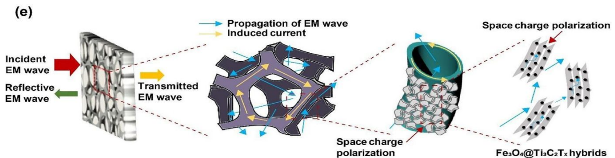
Fig.13: Schematic diagram of the EM waves absorption in \text{Fe}_3\text{O}_4@Ti_3C_2Tx/GF/PDMS composite. Reprinted with permission. Copyright (2020) [184]
