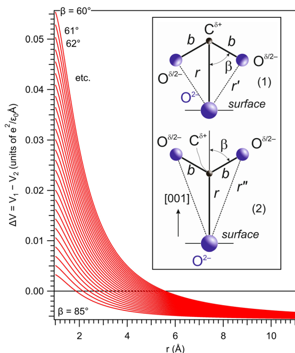
Fig. 8 The potential energy difference between the configuration with the oxygens from the bent CO 2 oriented towards the BTO(001) surface and that with the carbon closer to the BTO(001) surface. When this energy difference is positive, the molecule is supposed to be oriented with the carbon towards a surface oxygen anion.
