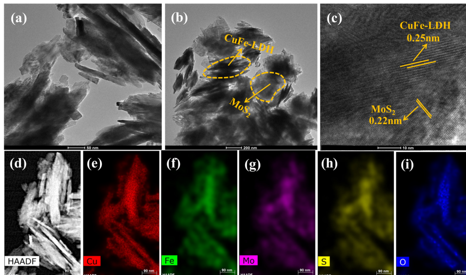
Fig. 2 TEM images of (a) CuFe-LDH, (b) CuFe-LDH/MoS 2 (20), (c) HR-TEM image of CuFe-LDH/MoS 2 (20) and (d)–(i) HAADF-STEM and elemental analysis of CuFe-LDH/MoS 2 (20).
