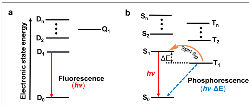
Fig. 8 (a) Emission mechanisms for doublet- and singlet/triplet-based organic emitters. Jablonski energy diagrams of the (a) doublet-quartet manifold, indicating doublet–doublet fluorescence. (b) Singlet–triplet manifold indicating singlet–singlet fluorescence, triplet–singlet phosphorescence, and spin flip processes, e.g., intersystem crossing (ISC, T_1 \rightarrow S_1 ) in TADF; triplet–triplet annihilation (TTA, 2 T_1 \rightarrow S_1 + S_0 ).
