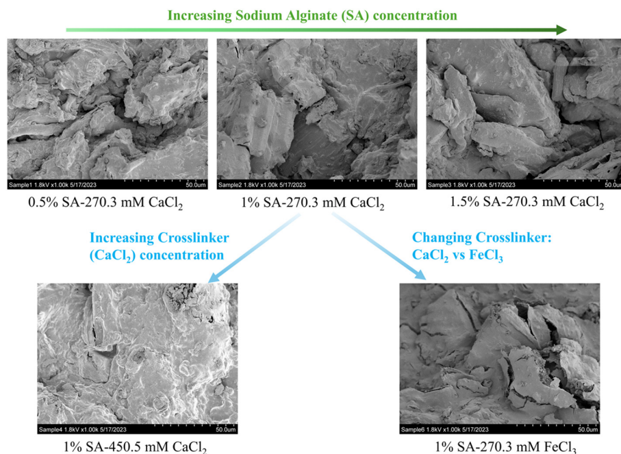
Fig. 3 Effects of varying bead compositions on the bead surface (SEM image scale bar = 50 \mu m). Increasing sodium alginate concentration smoothed the bead surface (crosslinker concentration was constant). Increasing the crosslinker concentration (3% to 5% CaCl 2 ) or changing the crosslinker to FeCl 3 from CaCl 2 also smoothed the bead surface (sodium alginate concentration was constant). Large cracks and pores were evident in beads crosslinked with FeCl 3 .
