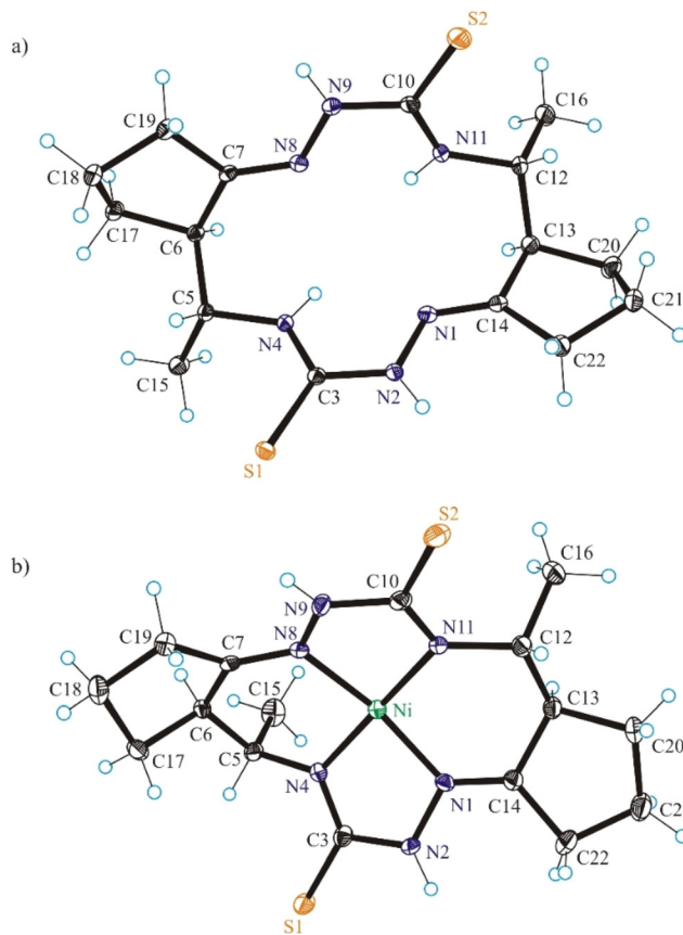
Fig. 1 ORTEP views of (a) H 2 L S and (b) Ni II L S as diastereomers with 5 R ,6 R ,12 R ,13 R -configuration. The thermal ellipsoids are drawn at 50% probability level. Selected bond distances (Å) and bond angles (°) in H 2 L S : N1–N2 1.3853(11), N2–C3 1.3662(11), C3–S1 1.6943(9), C3–N4 1.3316(12), N4–C5 1.4673(11), C5–C6 1.5491(13), C6–C7 1.5183(13), C7–N8 1.2806(11), N8–N9 1.3818(12), N9–C10 1.3723(12), C10–S2 1.6853(10), C10–N11 1.3294(13), N11–C12 1.4599(11), C12–C13 1.5439(15), C13–C14 1.5199(13), C14–N1 1.2780(12); \theta_{\text{N8-N9-C10-N11}} = 8.24(12) ; in Ni II L S : Ni–N1 1.854(3), Ni–N4 1.863(3), Ni–N8 1.871(2), Ni–N11 1.873(3), N1–N2 1.394(4), N2–C3 1.393(4), C3–S1 1.695(3), C3–N4 1.316(4), N4–C5 1.469(4), C5–C6 1.527(4), C6–C7 1.508(4), C7–N8 1.282(4), N8–N9 1.397(3), N9–C10 1.381(4), C10–S2 1.707(3), C10–N11 1.312(4), N11–C12 1.477(4), C12–C13 1.529(4), C13–C14 1.509(4), C14–N1 1.279(4); \theta_{\text{N1-N2-C3-N4}} = 12.5(4) , \theta_{\text{N8-N9-C10-N11}} = 6.4(4) .
