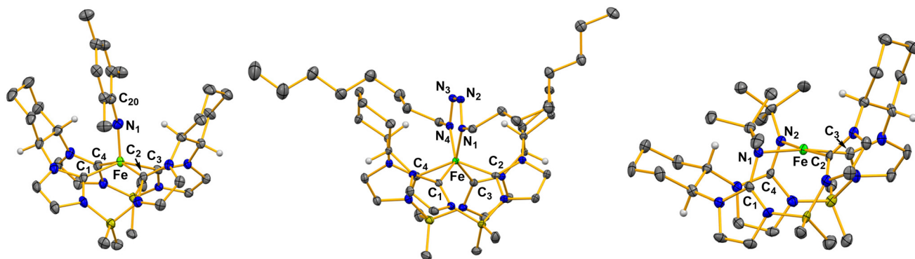
Fig. 2 X-ray crystal structures of (^{(S,S)}-1,2\text{-Cy, BMe}_2\text{TC}^H)\text{Fe}(\text{NMe}_s) ( 2 ), (^{(S,S)}-1,2\text{-Cy, BMe}_2\text{TC}^H)\text{Fe}(\text{n-octyl})\text{N}_4(\text{n-octyl}) ( 3 ), and (^{(S,S)}-1,2\text{-Cy, BMe}_2\text{TC}^H)\text{Fe}(\text{N}^t\text{Bu})_2 ( 4 ). Green, blue, grey, olive, and white ellipsoids (50% probability) represent Fe, N, C, B, and H atoms, respectively. Solvent molecules and H-atoms on non-stereogenic carbons are omitted for clarity.
