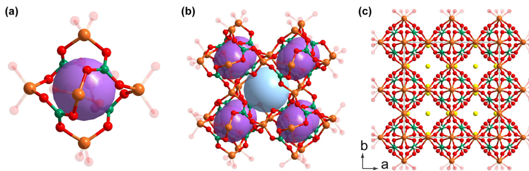
Fig. 3 (a) [\text{Ga}_6(\text{BO}_3)_4] cage. (b) Cubic cavity (blue ball) constructed from eight [\text{Ga}_6(\text{BO}_3)_4] cages (purple balls). (c) Structure of \text{Na}_4\text{Ga}_3\text{B}_4\text{O}_{12}(\text{OH}) . Na, Ga, B, O, and H are shown in yellow, orange, olive, and red, respectively.
