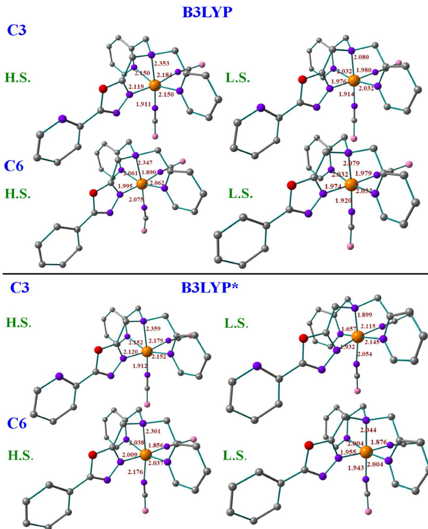
Fig. 6 Optimized structure with B3LYP & B3LYP* hybrid functional along with some selected bond parameters for complexes C3 and C6. Colour code: Orange = Fe (Iron), Purple = N (Nitrogen), Red = O (Oxygen), Grey = C (Carbon), Pink = B (Boron), and hydrogen atoms are omitted for clarity.
