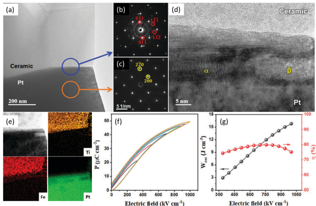
Fig. 13 (a) TEM micrograph of BF-ST-Nb-0.1BMN/Pt interface. (b) SAD pattern highlighting BF-ST-Nb-0.1BMN reflections. (c) SAD pattern from Pt area in (a). (d) High-resolution TEM micrograph showing different phases at ceramic/Pt interface. (e) Bright-field STEM image and EDS elemental maps of ceramic/Pt interface. (f) Unipolar P - E loops. (g) Energy storage properties ( W_{rec} and \eta ) for BF-ST-Nb-0.1BMN multilayer. 192 Reprinted (adapted) with permission from ref. 192 under the terms of the Creative Commons Attribution 3.0 Unported Licence, Royal Society of Chemistry.
