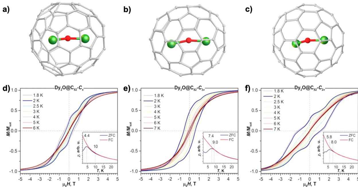
Fig. 6 Molecular structures of \text{Dy}_2\text{O}@C_s(6)\text{-C}_{82} (a), \text{Dy}_2\text{O}@C_{3v}(8)\text{-C}_{82} (b) and \text{Dy}_2\text{O}@C_{2v}(9)\text{-C}_{82} (c). Magnetic hysteresis curves of \text{Dy}_2\text{O}@C_s(6)\text{-C}_{82} (d), \text{Dy}_2\text{O}@C_{3v}(8)\text{-C}_{82} (e) and \text{Dy}_2\text{O}@C_{2v}(9)\text{-C}_{82} (f) in the range of 1.8–7 K using a field sweep rate of 2.9 \text{ mT s}^{-1} . The insets represent their corresponding ZFC/FC curves at an applied magnetic field of 0.2 T with a temperature sweep rate of 5 \text{ K min}^{-1} . Reproduced from ref. 102.
