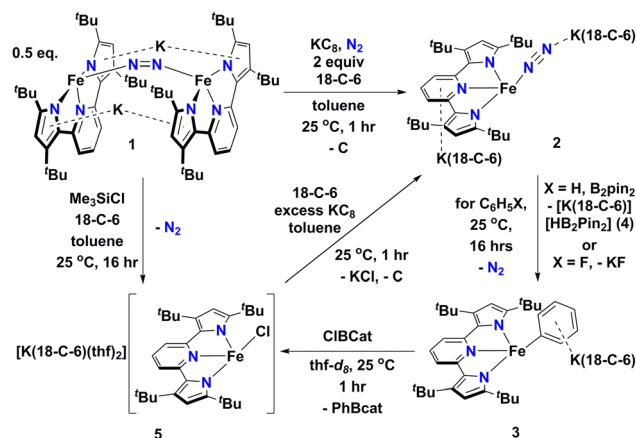
Scheme 1 Reaction scheme outlining formation and reactions of \{[K(18\text{-C-6})\}_2\{(t^{\text{Bu}}\text{pyrr}_2\text{pyr})\text{Fe}(N_2)\} (2).
