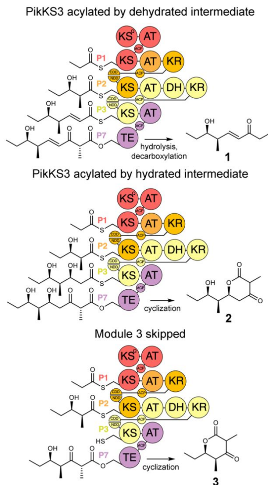
Fig. 2 Polyketide production by P1-P2-P3-P7 and variants. P1-P2-P3-P7 , engineered from the updated modules of the pikromycin synthase, synthesizes a β-ketoacid that spontaneously decarboxylates to the tetraketide olefin 1 . Tetraketide lactone 2 is generated when PikKS3 is acylated by the hydrated intermediate. Triketide lactone 3 is generated when the third module, P3 , is skipped.
