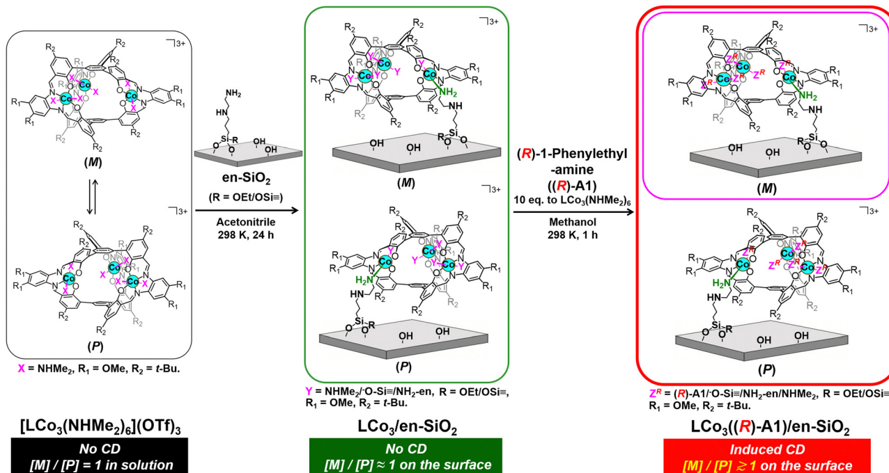
Scheme 1 Preparation of a supported helical LC 03 complex, LC 03 ((R)-A1)/en-SiO 2 , by grafting of [LC 03 (NHMe 2 ) 6 ](OTf) 3 on an ethylenediamine-functionalized SiO 2 surface ( en-SiO 2 ), followed by the addition of chiral ( R )-1-phenylethylamine. Possible paired surface structures are presented. The whole scheme for LC 03 (( R )-A1)/en-SiO 2 is presented in the ESI† (Scheme S1).
