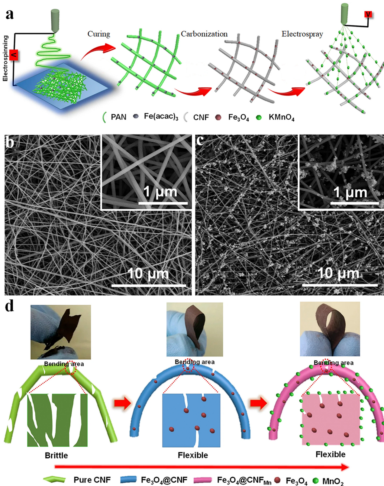
Fig. 12 (a) Schematics of flexible Fe 3 O 4 @CNFMn electrode preparation. (b and c) FE-SEM micrographs of the Fe 3 O 4 @CNF and Fe 3 O 4 @CNFMn fiber electrode respectively. (d) Photographs and mechanism of the enhanced flexibility of the Fe 3 O 4 @CNFMn electrode. Reproduced from ref. 108 with permission from Nature, copyright 2017.
