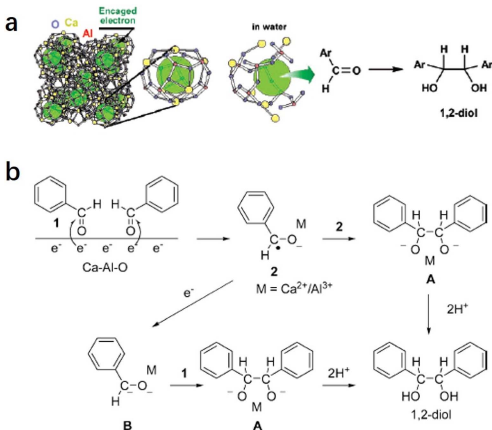
Fig. 13 (a) The C12A7:e - electrode was employed for a pinacol coupling reaction in aqueous media. The Ca–Al–O gel formed by the destruction of the crystal structure of the C12A7:e - by water media played a key role in transferring the electron to electrophilic aldehydes. (b) Scheme of a possible mechanism for pinacol coupling mediated by C12A7:e - . Copyright 2007, American Chemical Society.
