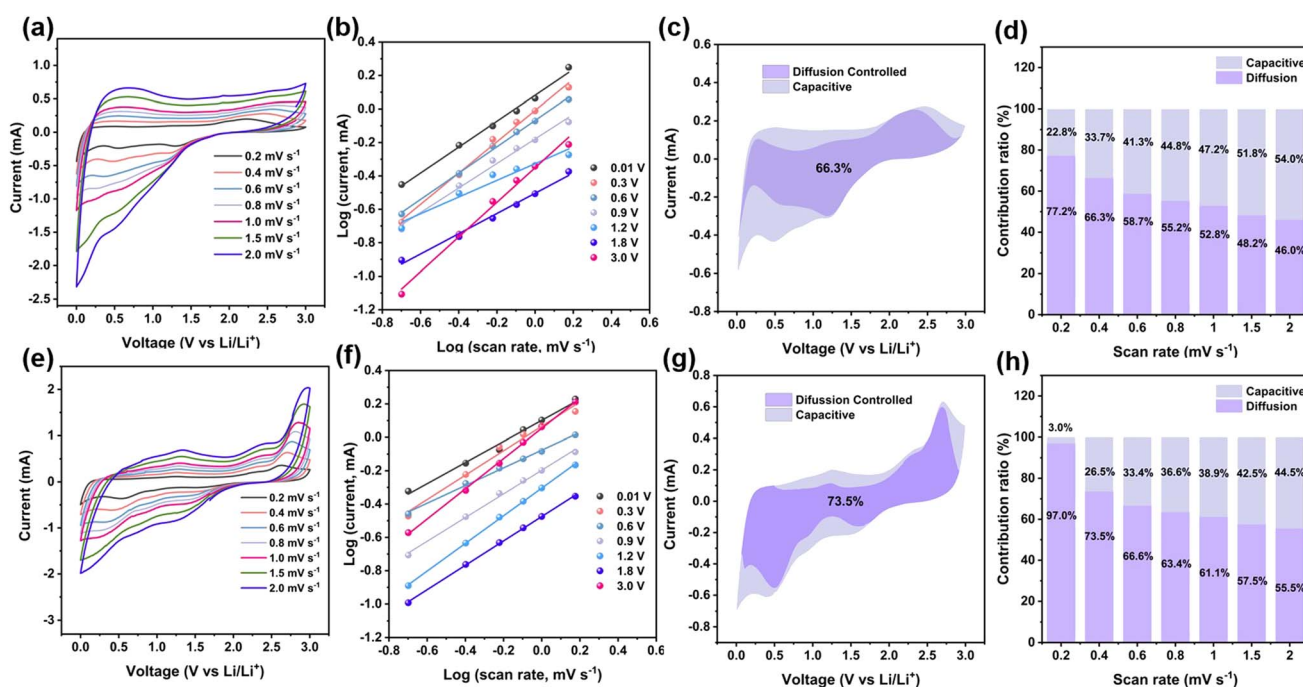
Fig. 7 (a and e) CV curves of the as-prepared VSe 2 -ZrO 2 /C/MXene and after cycling for 250 cycles at different scan rates. (b and f) Linear relationship between \log(i) and \log(\nu) at different voltages for the as-prepared VSe 2 -ZrO 2 /C/MXene and after cycling for 250 cycles. (c and g) Separation of capacitive and diffusion-controlled contribution areas at 0.4 \text{mV s}^{-1} for the as-prepared VSe 2 -ZrO 2 /C/MXene and after cycling for 250 cycles. (d and h) Ratios of capacitive and diffusion-controlled contributions at different scan rates for the as-prepared VSe 2 -ZrO 2 /C/MXene and after cycling for 250 cycles.
