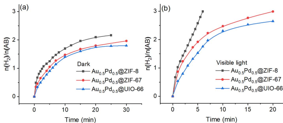
Fig. 3 AB methanolsis catalyzed by Au 0.5 Pd 0.5 on different supports: (a) in the absence of light and (b) in the presence of visible light. Reaction conditions: 1 mmol AB; 1.25% mmol MNP; temperature: 25 ± 0.5 °C.
