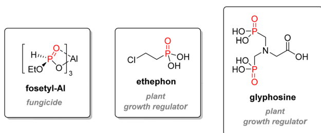
Fig. 22 Examples of organophosphorus agrochemicals.
