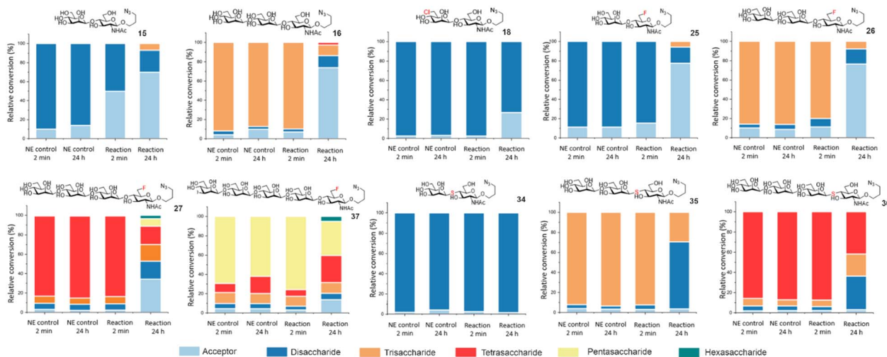
Fig. 4 Phosphorolysis of Manβ1,4-GlcNAc-N 3 analogues, with relative conversions determined by ITag LC-MS analysis. NE denotes: no enzyme control.
