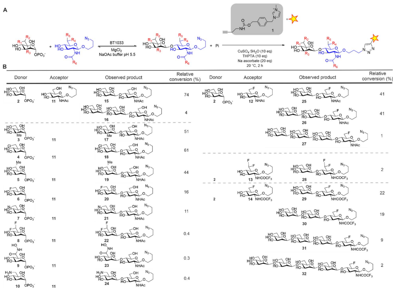
Fig. 2 (A) ITag screening methodology for BT1033 reactions. Reaction mechanism depicted in reverse phosphorylase direction. (B) BT1033 activity towards unnatural donors and acceptors. 3,15
