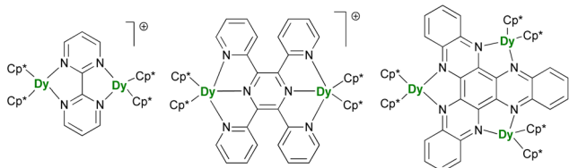
Fig. 9 Molecular structures of [[(\text{Cp}^*)_2\text{Dy}]_2(\mu\text{-bipym})]^+ , 196 [[(\text{Cp}^*)_2\text{Dy}]_2(\mu\text{-tppz})]^+ , 197 and (\text{Cp}^*)_6\text{Dy}_3(\mu_3\text{-HAN}) . 198
