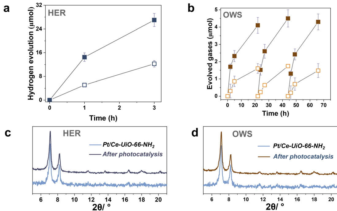
Fig. 7 (a) Photocatalytic HER using Ce-UiO-66-NH 2 (empty square) or Pt/Ce-UiO-66-NH 2 (filled square) and, (c) the corresponding PXR D pattern of Pt/Ce-UiO-66-NH 2 before and after catalysis. (b) Photocatalytic overall water splitting (OWS) into H 2 (filled square) and O 2 (emptied square) using Pt/Ce-UiO-66-NH 2 and, (d) the corresponding PXR D patterns of Pt/Ce-UiO-66-NH 2 before and after photocatalytic recycling. Reaction conditions: photocatalyst amount (20 mg), water (20 mL), simulated sunlight irradiation (150 W Hg–Xe lamp equipped with an AM 1.5G filter), 35 °C.
