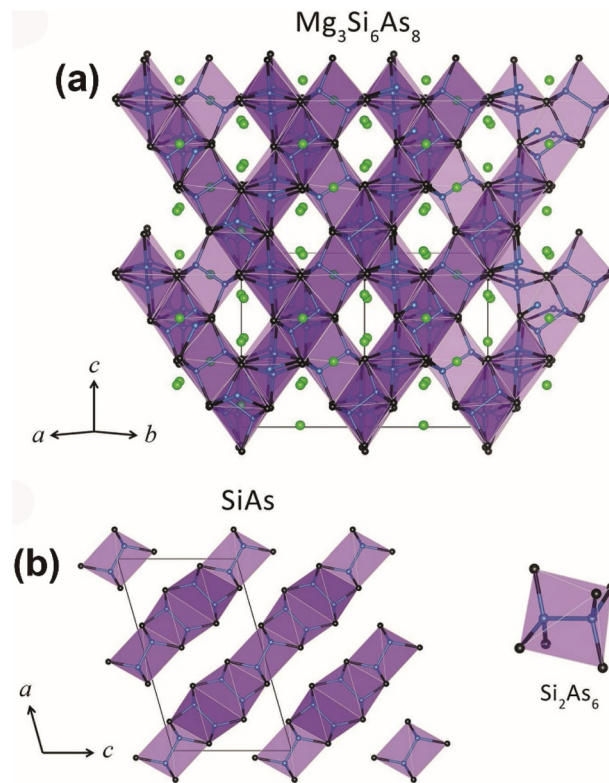
Fig. 3 (a) Crystal structure of the 3D Si–As network in \text{Mg}_3\text{Si}_6\text{As}_8 and (b) SiAs with \text{Si}_2@\text{As}_6 marked as purple octahedra. Green atom: Mg; blue atom: Si; black atom: As. Copyright 2018 Wiley.
