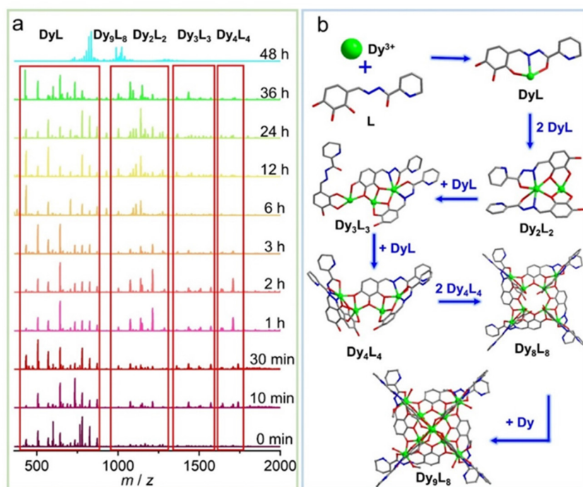
Fig. 3 Time-correlated HRESI-MS spectrum of cluster 1 (a) and schematic of the possible assembly mechanism of cluster 1 (b).
