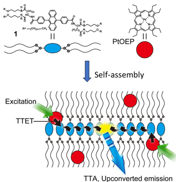
Fig. 4 A self-assembled network of acceptor [10 mM] and entrapped donor molecules [10 \mu M], leading to extremely efficient TET and TTA processes enhancing the \Phi_{UC} up to 30%. Adopted with permission from ref. 34. Copyright 2015 Springer Nature.
