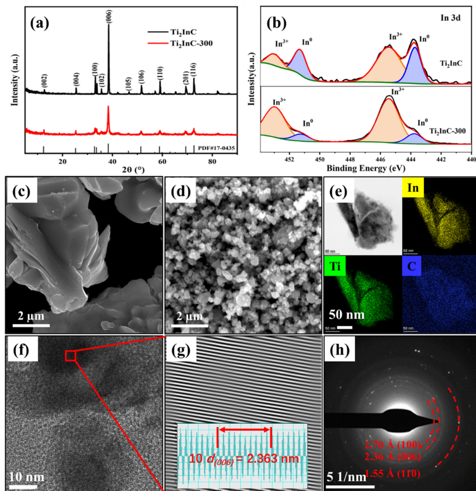
Fig. 1 (a) XRD patterns of the Ti 2 InC and the Ti 2 InC-300. (b) In 3d XPS spectra of Ti 2 InC and Ti 2 InC-300. (c) and (d) SEM images for Ti 2 InC and Ti 2 InC-300, respectively. (e) TEM morphology and the distribution of the corresponding elements. (f) HRTEM morphology and (g) the corresponding IFFT image of the area marked with a red rectangle in (f). (h) The SAED pattern of the Ti 2 InC-300.
