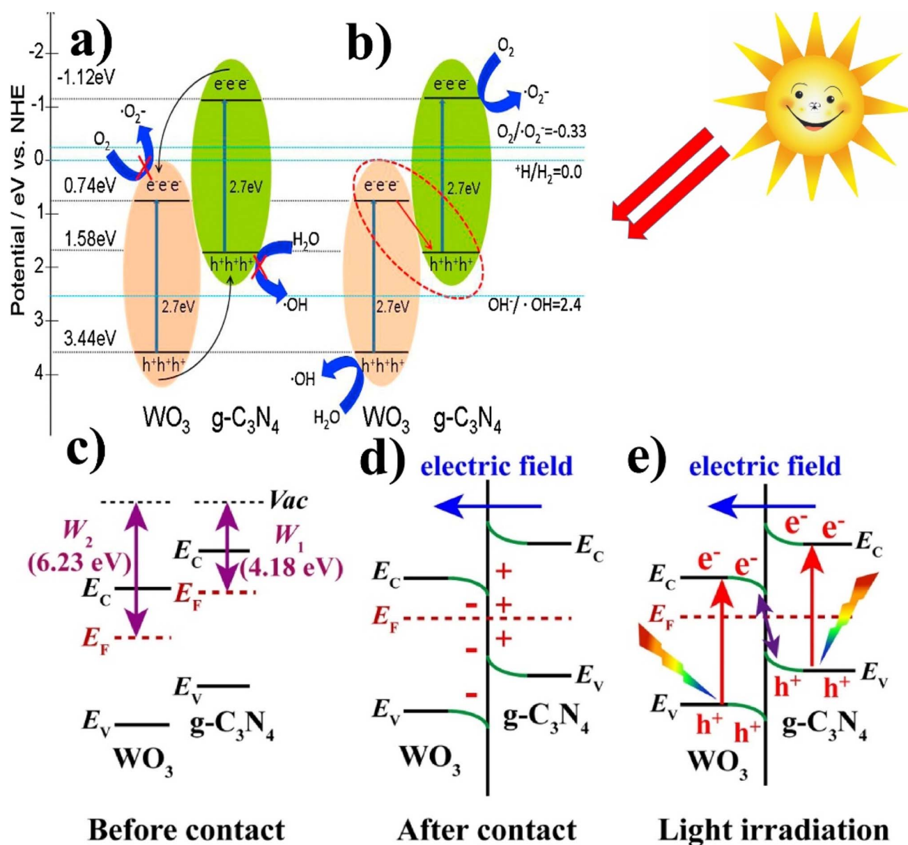
Fig. 11 (a and b) Generalized mechanism of the photoexcited e^-/\text{h}^+ separation process of \text{WO}_3/\text{g-C}_3\text{N}_4 (reproduced with permission from ref. 116 Copyright 2014, Elsevier). (c) Before contact with the work functions, \text{g-C}_3\text{N}_4 and \text{WO}_3 ; (d) after contact at the internal electric field/band edge bending at the interface of \text{WO}_3/\text{g-C}_3\text{N}_4 . (e) Under light irradiation, the S-scheme charge transfer mechanism between \text{WO}_3 and \text{g-C}_3\text{N}_4 (reproduced with permission from ref. 82 Copyright 2018, Elsevier).
