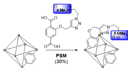
Scheme 1 Strategical installations of aromatic and aliphatic quaternary ammonium groups into MOFs via PSM and PSE processes.
