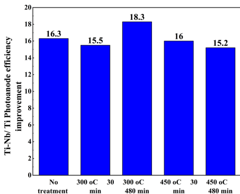
Fig. 19 The conversion efficiency of DSSCs using Ti-Nb photoanodes with and without H 2 O 2 treatment after annealing at (a) 300 °C and (b) 450 °C for 30 and 480 min and (c) the improvement in efficiency percentage of Ti-Nb compared to Ti photoanodes. 175
