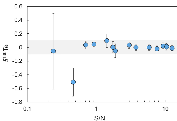
Fig. 2 Plot of \delta^{130}\text{Te} for mixtures of the Te double spike with the London Te standard solution at varying S/N values. The shaded area denotes the within day precision of 0.1\% (2SD).
