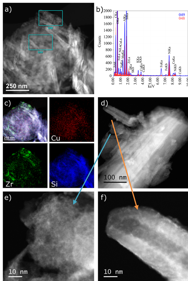
Fig. 2 (a) Overview HAADF-STEM image, (b) EDX spectra from regions marked in (a), (c) EDX elemental maps of CuZr/5A, (d) more detailed HAADF-STEM image with Zr containing regions highlighted in (c), showing a rather large amorphous particle, and (f), showing bright smaller clusters adhering to the support surface.
