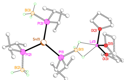
Fig. 1 Molecular structure of 2Li with C-bound H atoms omitted for clarity. Selected bond lengths (Å) and angles (°): Sn(1)–P(2) 2.6349(6), Sn(1)–P(1) 2.6219(6), Sn(1)–P(3) 2.6241(6), P(1)–B(1) 1.956(3), P(2)–B(2) 1.957(3), P(3)–B(3) 1.957(3), Li(1)–B(1) 2.381(5), Li(1)–O(1) 1.916(5), Li(1)–O(2) 1.926(5), Li(1)–O(3) 1.955(5), P(1)–Sn(1)–P(2) 103.459(19), P(1)–Sn(1)–P(3) 103.853(18), P(2)–Sn(1)–P(3) 104.400(19).
