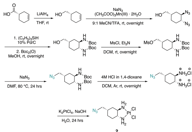
Fig. 2 Synthesis of 2 .
