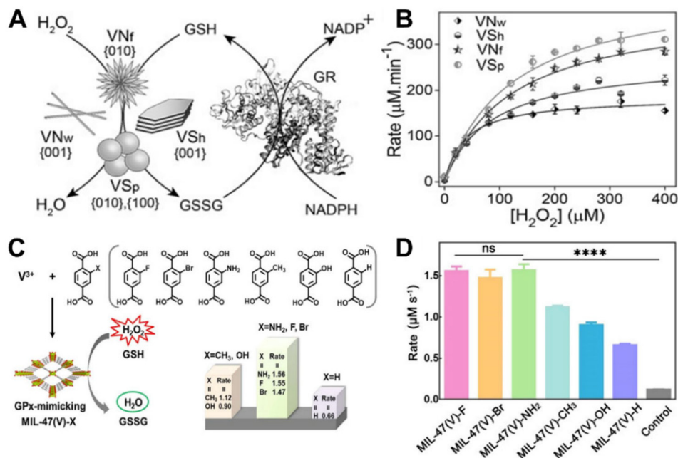
Fig. 6 (A and B) GPx-like activities of different \text{V}_2\text{O}_5 . Adapted with permission from ref. 46. Copyright (2018) John Wiley and Sons. (C and D) A schematic of the synthesis of MIL-47(V)-X MOFs and their GPx-like activities. Adapted with permission from ref. 48. Copyright (2021) John Wiley and Sons.
