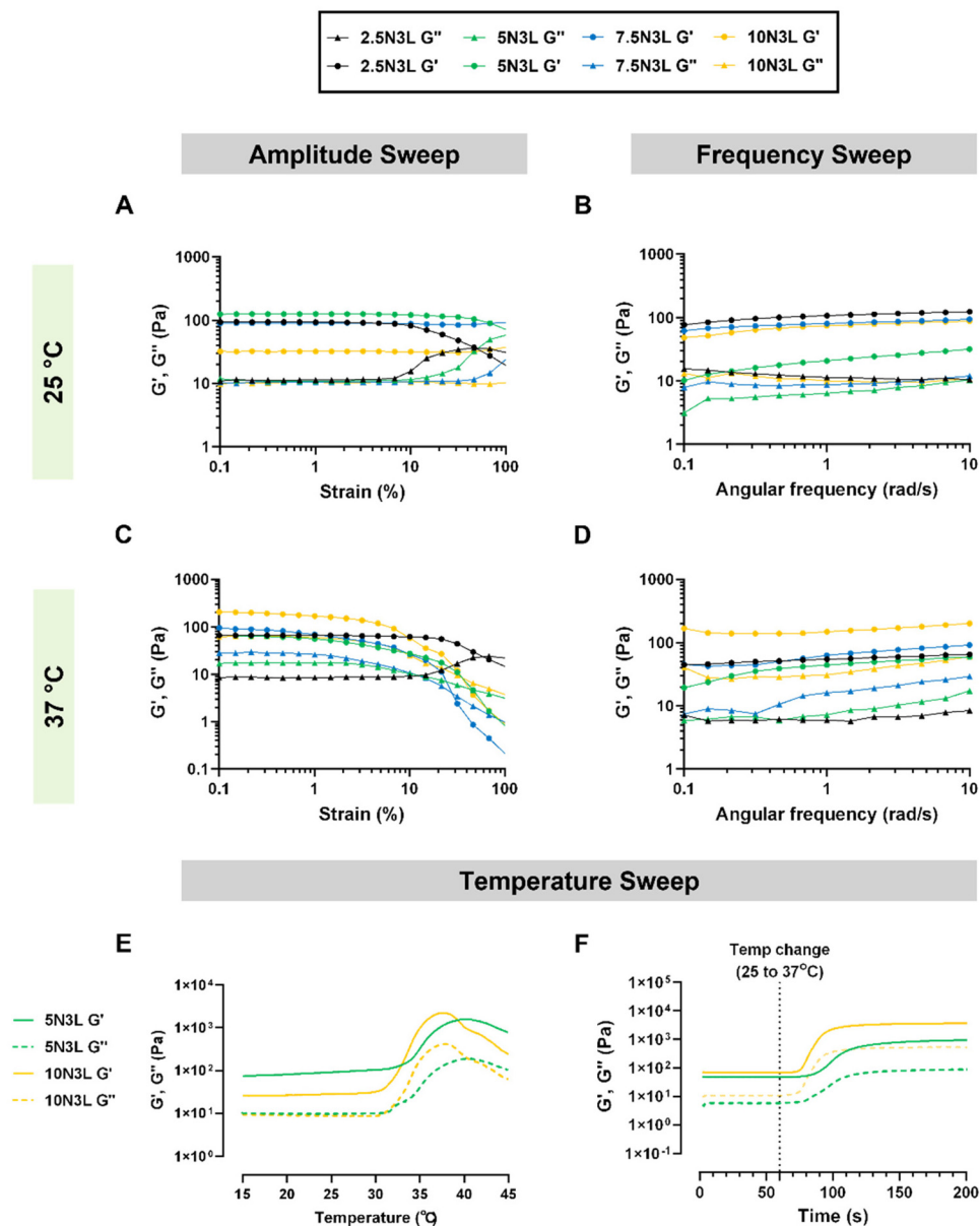
Fig. 2 Representative (A) amplitude sweep, and (B) frequency sweep of our p(NIPAM) and LAPONITE®-based T-STH at 25 °C. Representative (C) amplitude sweep, and (D) frequency sweep of our T-STH at 37 °C. The amplitude sweep was used to determine the linear viscoelastic range (LVER). The frequency sweeps were performed at 1% strain in the LVER of the T-STHs. Temperature-dependent change in G' and G'' values of our p(NIPAM) and LAPONITE®-based T-STHs (E) as the temperature slowly ramps up from 15 °C to 45 °C, and (F) as the temperature is suddenly changed from 25 °C to 37 °C.
