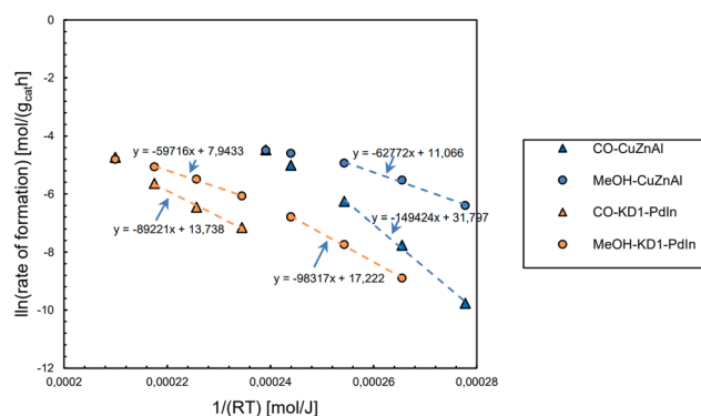
Fig. 12 Performance of selected catalysts in terms of the rate of production versus the input energy in the FReSMe project. 89
