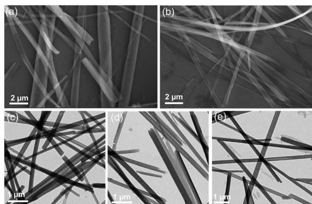
Fig. 5 SEM images of nanostructures formed in DMSO solutions of (a) Cs^+[Eu(+-tfac)_4]^- and (b) Na^+[Eu(+-tfac)_4]^- . TEM images of the self-assembled aggregates formed from (c) Cs^+[Eu(+-tfac)_4]^- , (d) Rb^+[Eu(+-tfac)_4]^- and (e) K^+[Eu(+-tfac)_4]^- .
