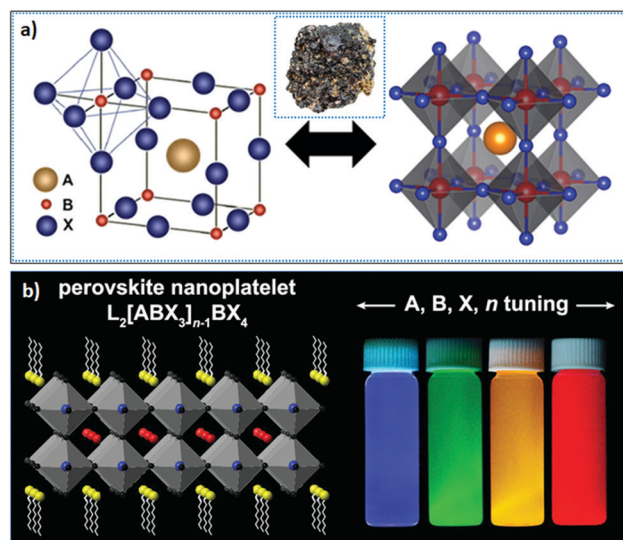
Fig. 1 (a) Bulk structure of perovskites; the inset shows the perovskite mineral \text{CaTiO}_3 ; and (b) layered 2D perovskite ( n = 2 ) (left), where the emission color can be tuned upon varying X or n (right). panel (a) reprinted with permission from ref. 65. Copyright 2016 American Chemical Society. Panel (b) reprinted with permission from ref. 66 Copyright 2021 Elsevier.
