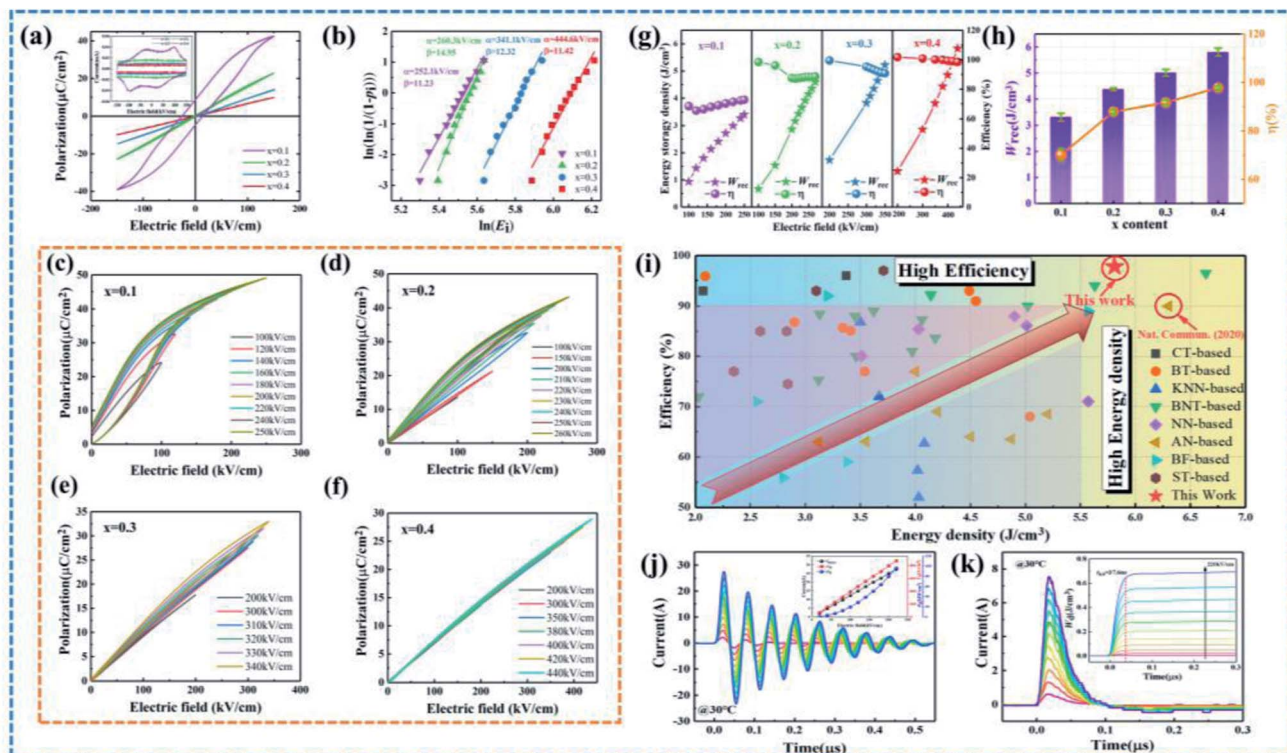
Fig. 3 (a) Bipolar P - E loops and I - E curves measured at 150 \text{ kV cm}^{-1} and room temperature and (b) Weibull distributions for BNT-BAT- x CT ceramics; unipolar P - E loops measured at 10 Hz: (c) x = 0.1 , (d) x = 0.2 , (e) x = 0.3 , and (f) x = 0.4 ; (g) electric field-dependent variation of W_{\text{rec}} and \eta ; (h) change of W_{\text{rec}} and \eta under respective E_b for BNT-BAT- x CT ceramics; (i) a comparison of ESP among the x = 0.4 ceramic and other recently reported dielectric ceramics; (j) underdamped and (k) overdamped discharge waveforms in different electric fields for the x = 0.4 sample, insets show the variation of I_{\text{max}} , C_D and P_D values and the calculated W_d curves.
