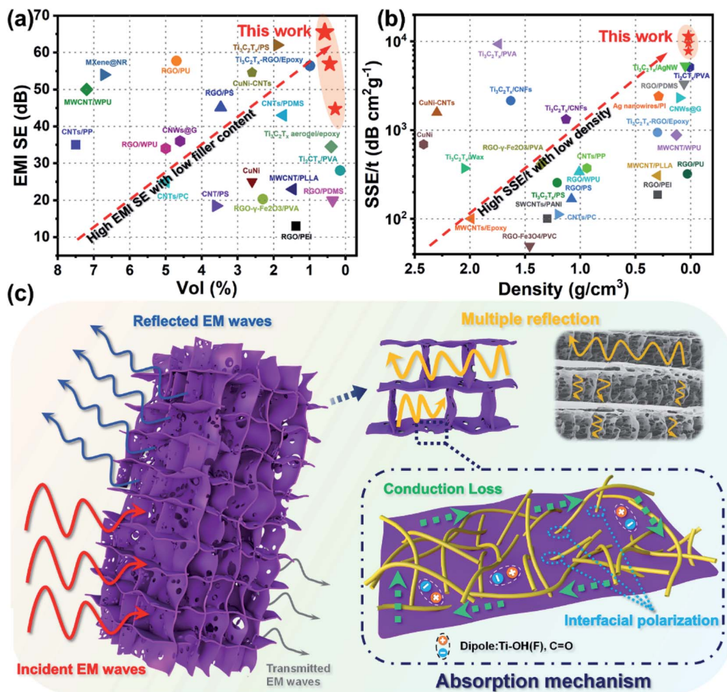
Fig. 6 (a) EMI SE versus \text{Ti}_3\text{C}_2\text{T}_x content (vol%) and (b) SSE/ t versus density of the anisotropic \text{Ti}_3\text{C}_2\text{T}_x/\text{ANF} aerogels compared with previous reports. (c) Electromagnetic shielding mechanism of the anisotropic \text{Ti}_3\text{C}_2\text{T}_x/\text{ANF} aerogel.
