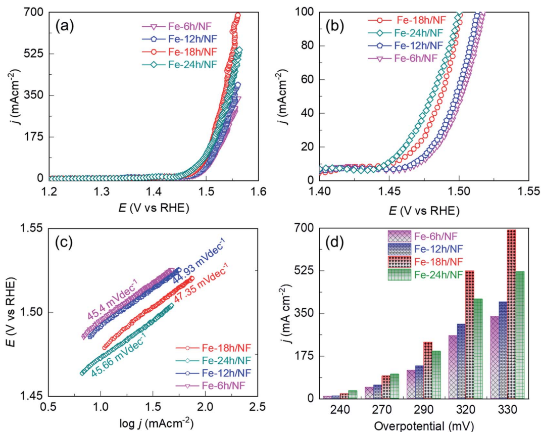
Fig. 3 Comparison of the electrocatalytic performance of the etched NF in a 1 M KOH solution: iR compensated anodic linear sweep voltammograms (LSVs) of the (a) NFs etched for 6, 12, 18, and or 24 h, (b) magnified view of (a) below 100 mA cm -2 , (c) corresponding Tafel slopes extracted from the LSVs, and (d) current density profiles with respect to the OER overpotential.
