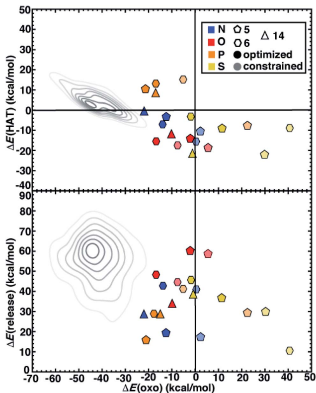
Fig. 6 \Delta E(\text{oxo}) vs. \Delta E(\text{HAT}) (top) and \Delta E(\text{oxo}) vs. \Delta E(\text{release}) (bottom) reaction energetics (in \text{kcal mol}^{-1} ) of representative TMCs from prior work 22 compared to 5-membered (pentagons) and 6-membered (hexagons) ring SAC models along with 14-membered macrocyclic Fe complexes (triangles). The SACs and macrocycles are colored by the metal-coordinating atoms in the ligands, as indicated in inset legend. The TMCs from prior work are the full low-spin Fe(II) subset from the square pyramidal constrained (SQ) set of ref. 22. The kernel density estimates of the distributions for the TMC set are colored in gray and shown as contour lines with decreasing saturation in 7 evenly spaced levels. The SACs are distinguished by full geometry optimization (opaque) and constrained optimization (translucent).
